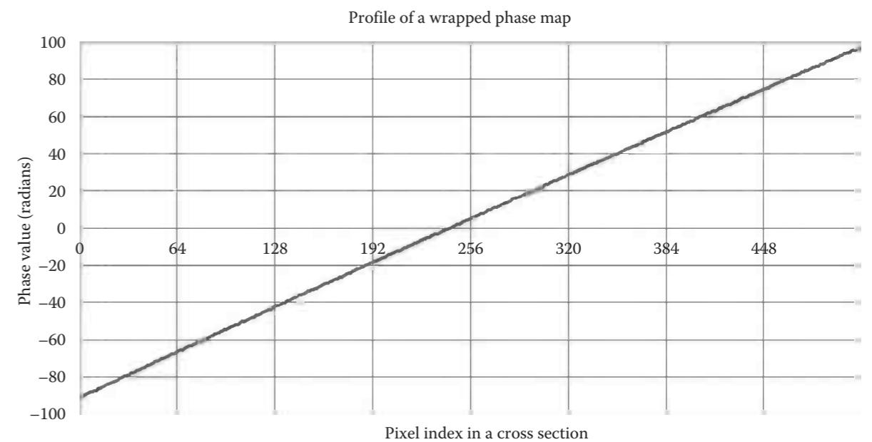
FIGURE 7.9 Profile of an unwrapped phase map without 2\pi discontinuity.
